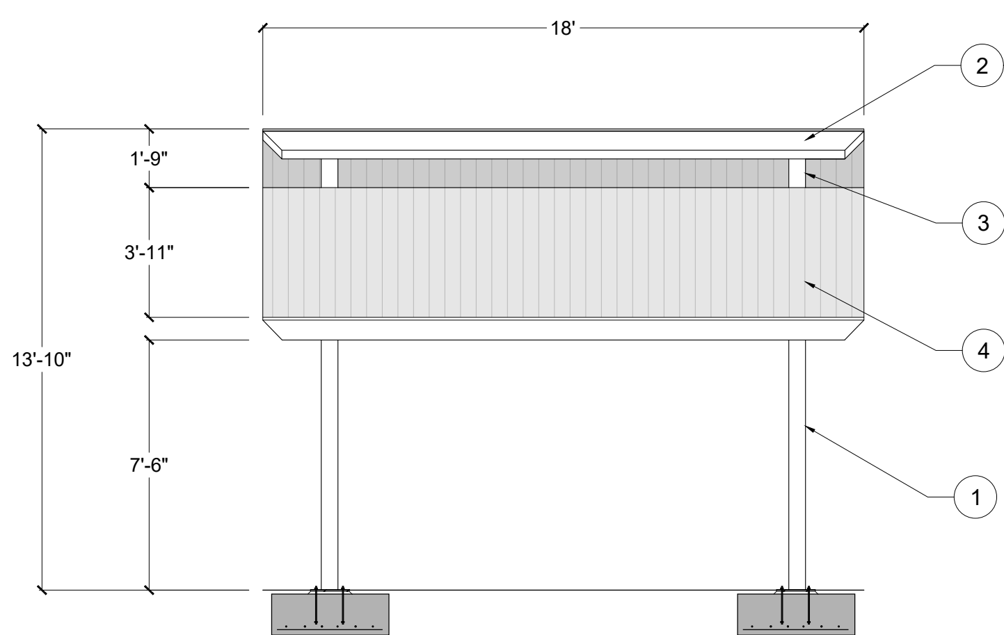
2 SIDE ELEVATION SCALE 1/4" = 1'
